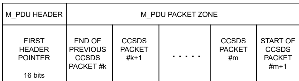
Figure 4-3: Multiplexing Protocol Data Unit (M_PDU)
